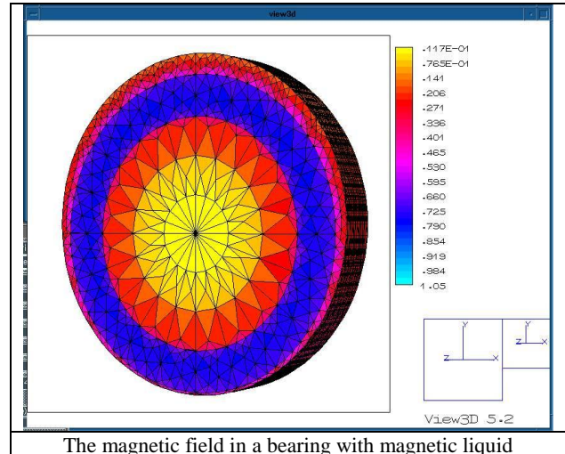
The magnetic field in a bearing with magnetic liquid
