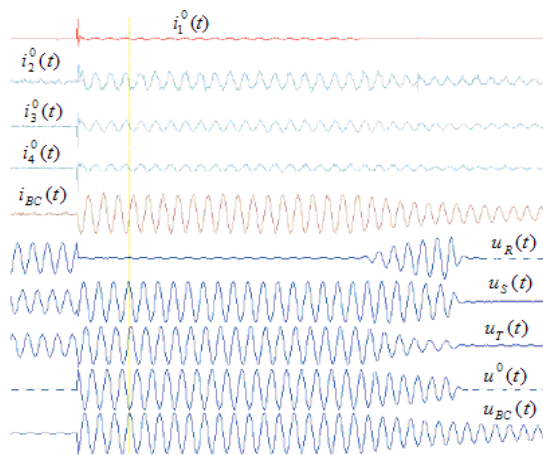
Time variation of the phase voltages and zero sequence current for the phase-to-ground when the network is in resonant regime
