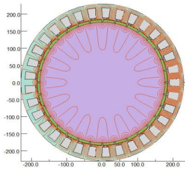
Magnetic field lines distribution
