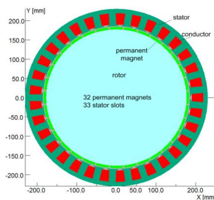
The analyzed PM wind generator
